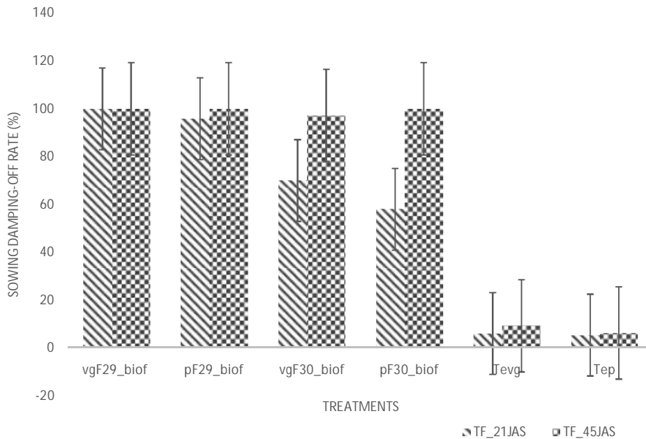
Figure 2. Histogram of damping-off rates according to treatments
