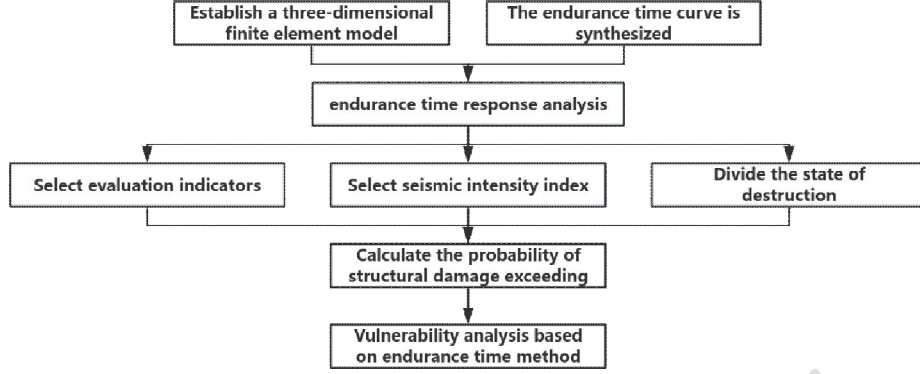
FIG. 2 Flowchart of vulnerability analysis based on endurance time method
