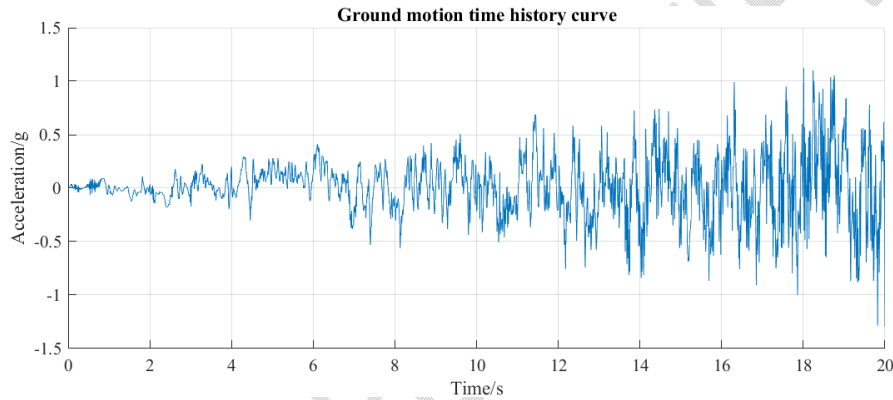
FIG. 1 Seismic time-history acceleration curve
