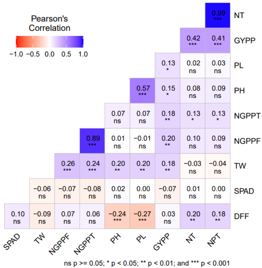
Figure-2: Correlation analysis among yield and yield component traits in rice
