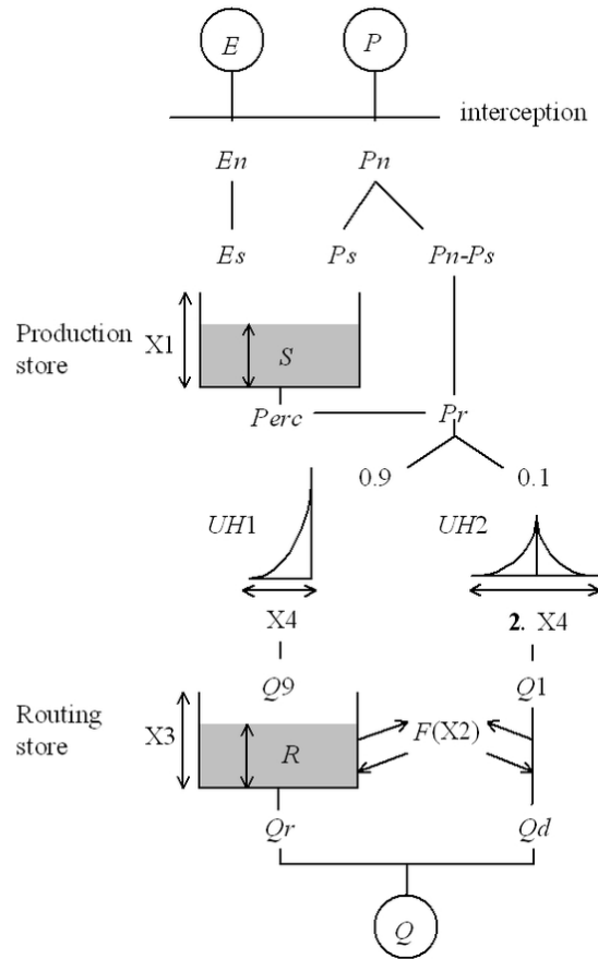
Fig. 3. Diagram of the GR4J rainfall-runoff model [23]
