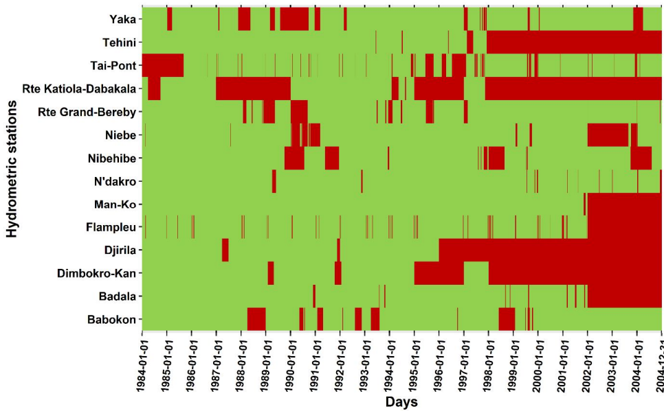
Fig.2. Availability of flow data over 1984-2004 period. Missing data are plotted in red, whereas available data are shown in green.
