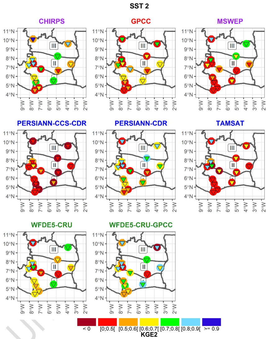
Fig.6. Spatial representation of KGE2 values obtained from calibration and validation in SST2.
