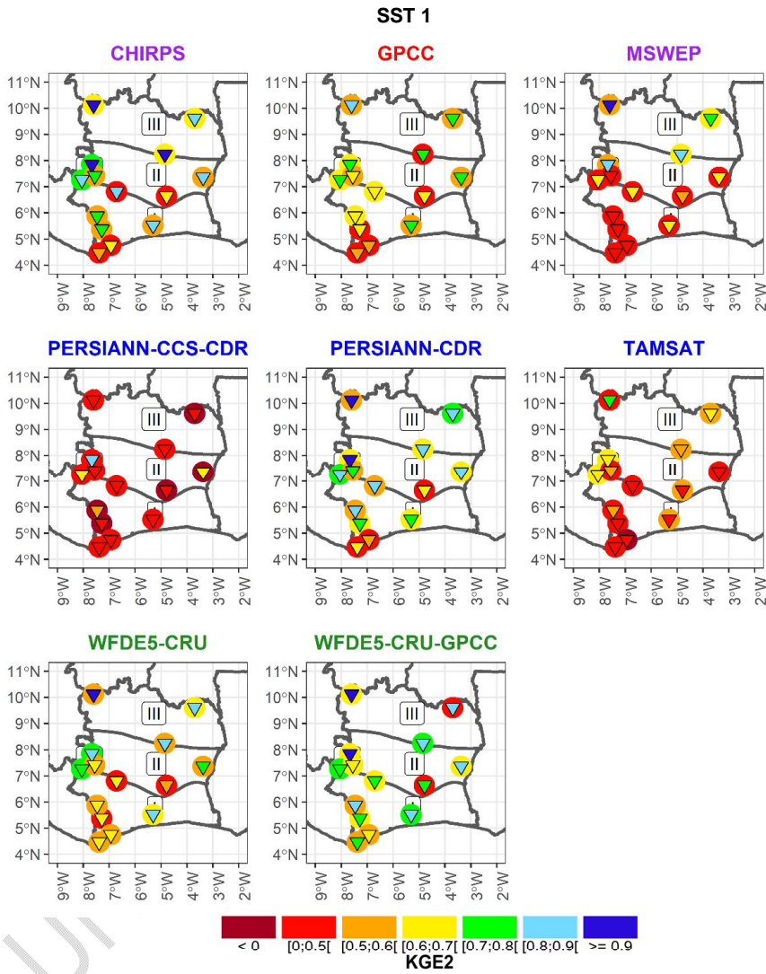
Fig.5: Spatial representation of KGE2 values obtained from calibration and validation for SST1.
