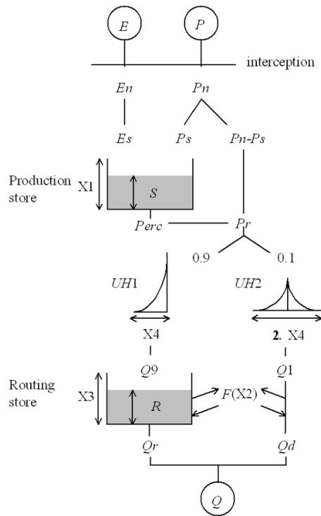
Fig. 3. Diagram of the GR4J rainfall-runoff model [23]
