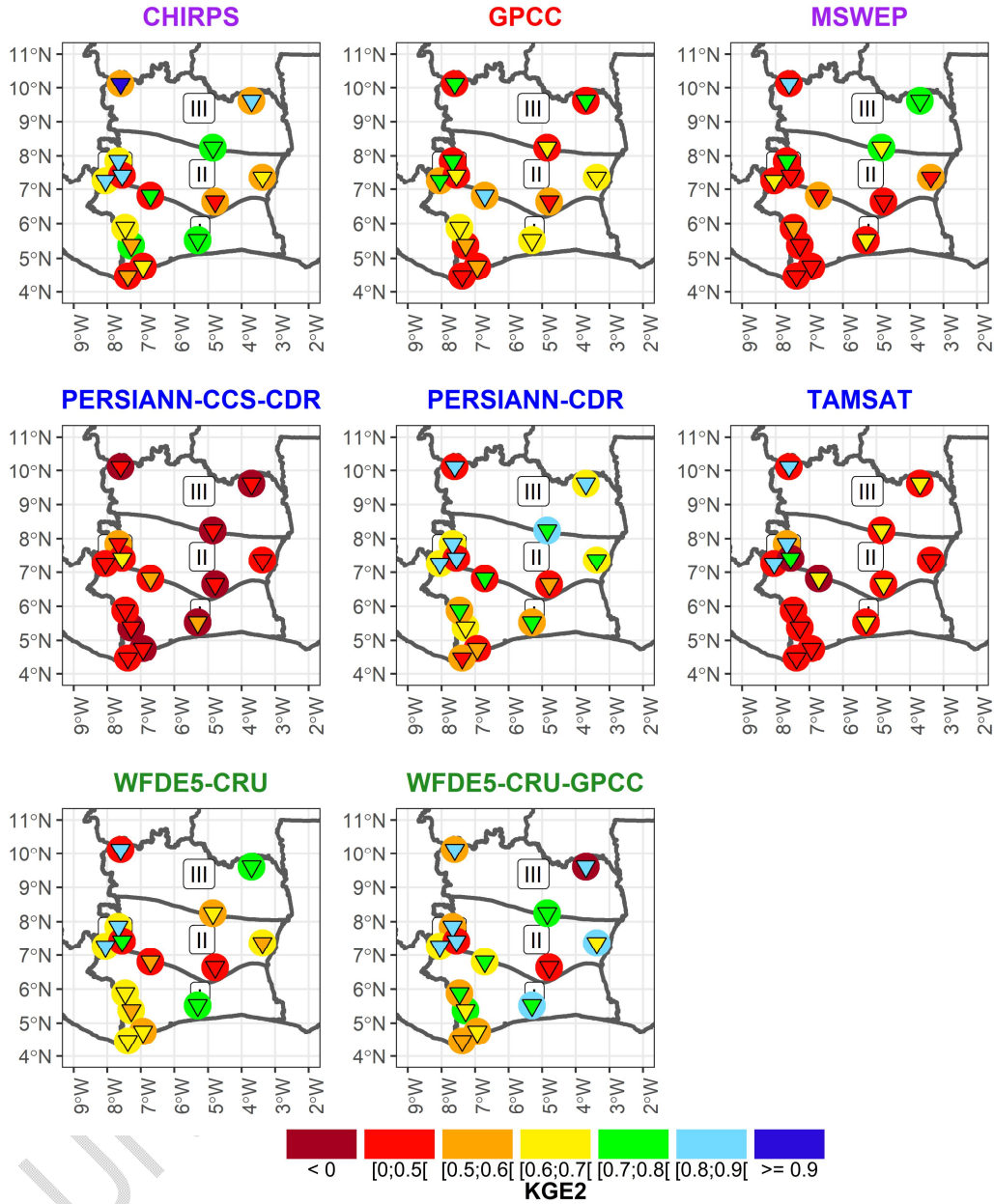
Fig.6. Spatial representation of KGE2 values obtained from calibration and validation in SST2.
