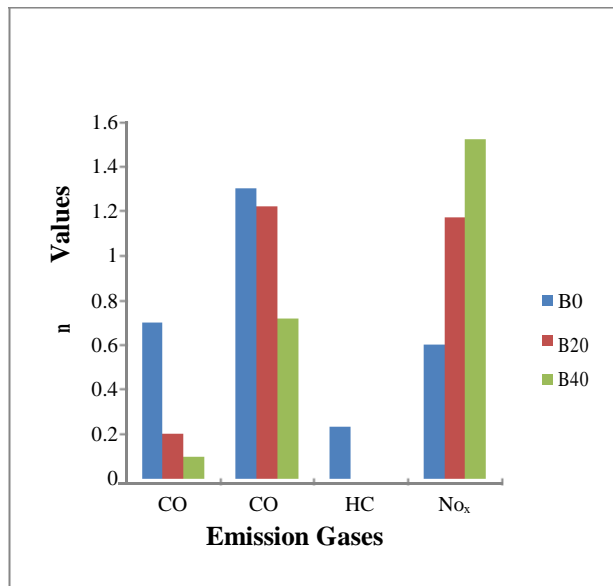
Figure 3: Emission Characteristics of Soyabean oil at a speed of 1600rpm
