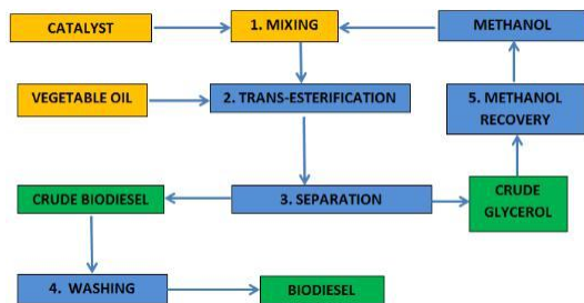
Fig 1: Soyabean oil transesterification process
