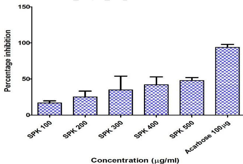
Fig 1. Percentage inhibition of test drug SPK and Standard on Alpha Amylase Enzyme Inhibition Assay
