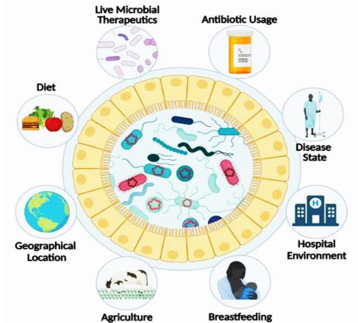
Fig. 1. The description of the factors that affect the resistome. Taken after Crits-Christoph et al. (2022)[58].
