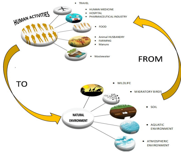
Fig. 2. Description of the reservoir of ARGs. Taken after Cuadrat et al. (2020) [66].
