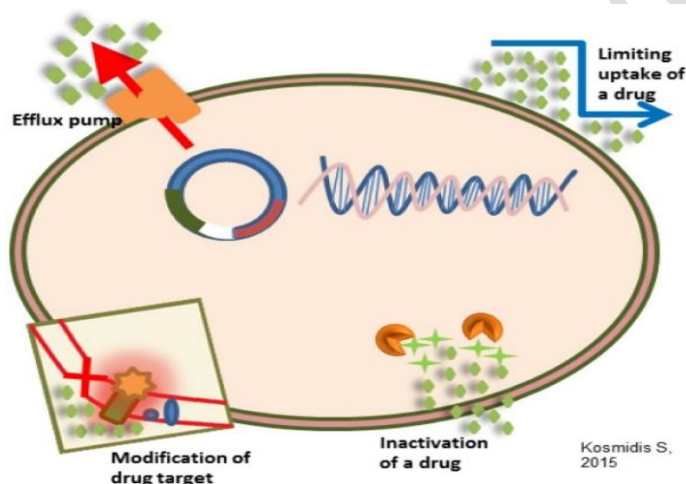
Fig. 4. Types of antimicrobial resistance mechanisms in bacteria. Taken after Munita and Arias (2016)[16].
