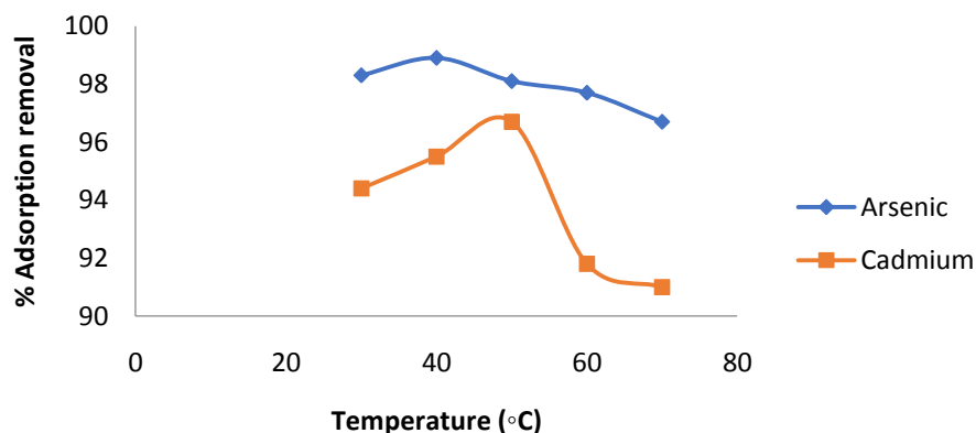
Fig. 10: Effect of temperature
