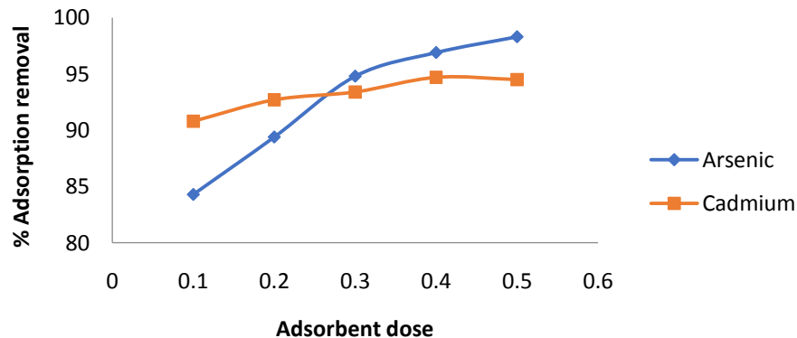
Fig. 8: Effect of adsorbent dose
