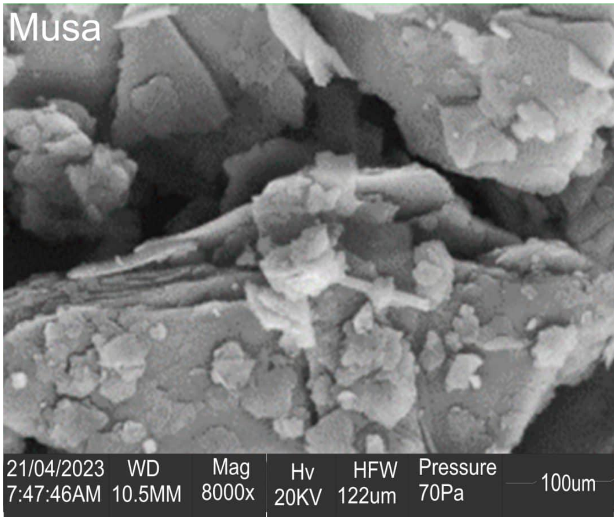
Fig. 4: SEM of the impregnated MHFS
