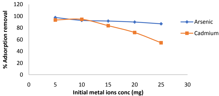
Fig. 7: Effect of initial concentration
