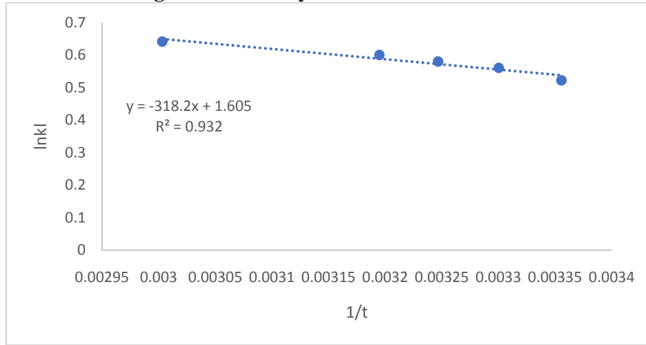
Fig. 21: Thermodynamic on Cd for MHFS
