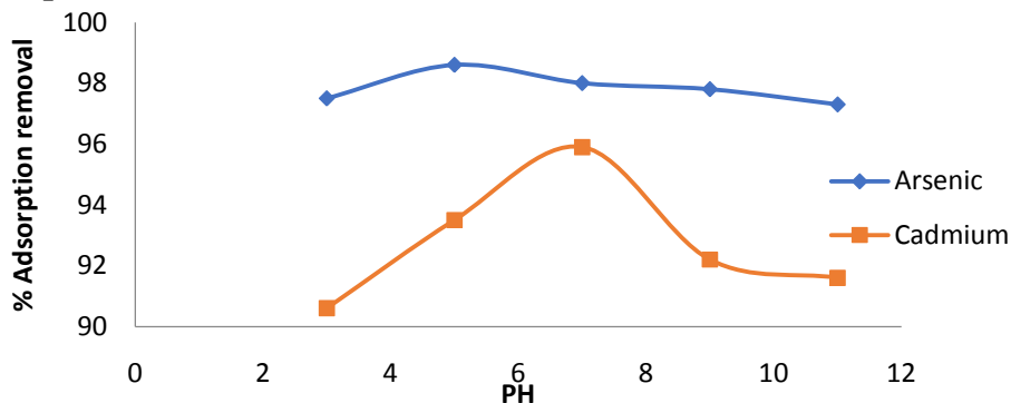
Fig. 9: Effect of pH
