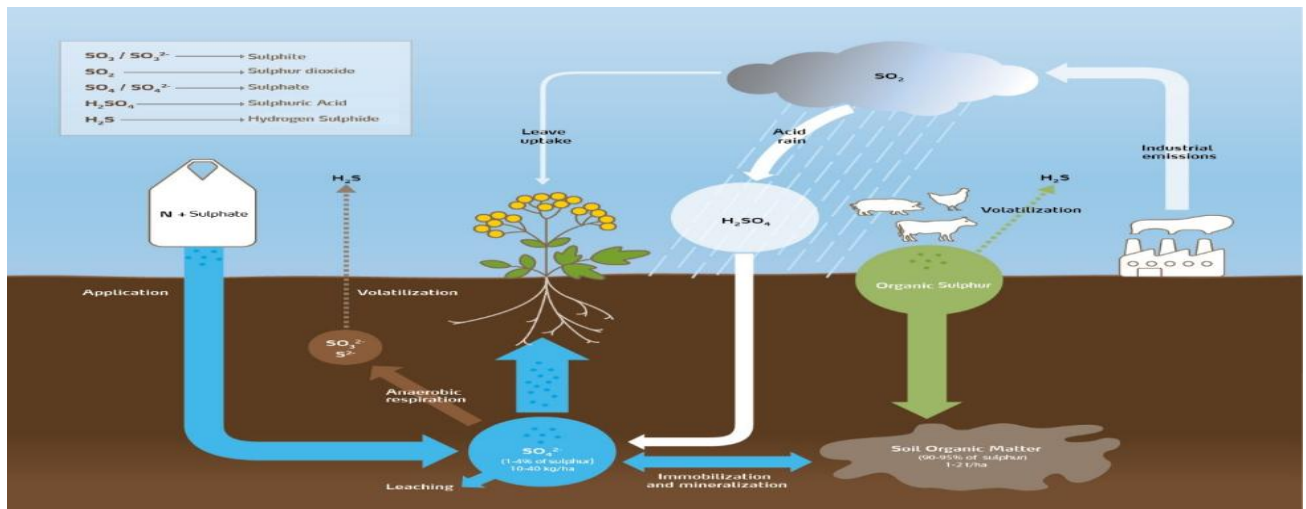
Fig 1: Sulphur Cycle
