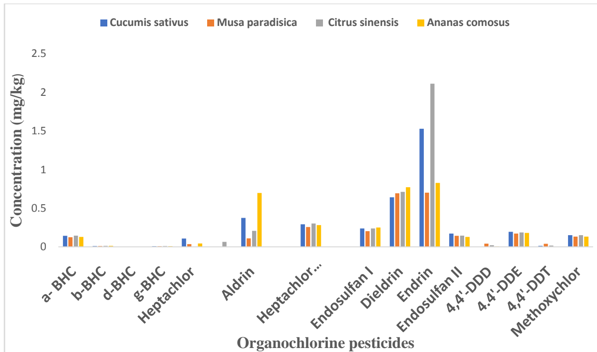
Fig.2: Concentration of Organochlorine pesticides (OCP) in Fruits from Odoluwa Central Market Ile Oluji
