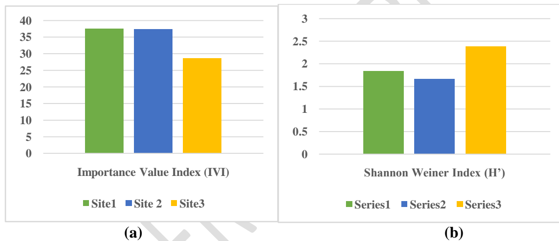
Fig 4: The Importance Value Index, IVI (a), and Shannon Weiner's Index, H' (b) of all the 3 sites
