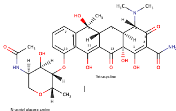
Figure 2 The chemical structure of the glycosylated tetracycline
