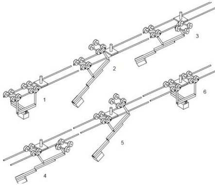
Fig .2 .Expliner robot crossing obstacles
