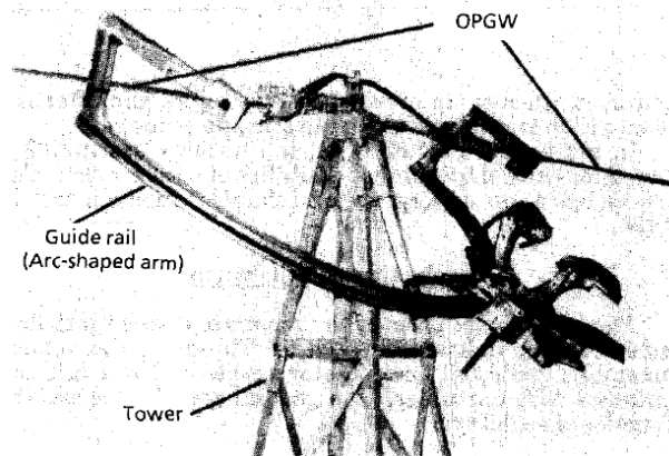
Fig. 1. Robot crossing the tower diagram
