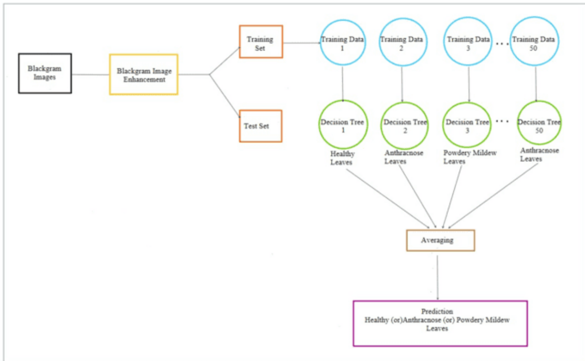
Figure 3. Random Forest Classifier for Blackgram images
