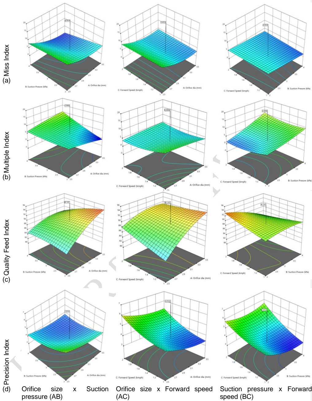
Fig.2 Comparison of different performance indices (level of significance, 5%): (a) miss index; (b) multiple index; (c) quality of feed index (d) Precision index for Orifice size x Suction pressure (AB), Orifice size x Forward speed (AC) , Suction pressure x Forward speed (BC).
