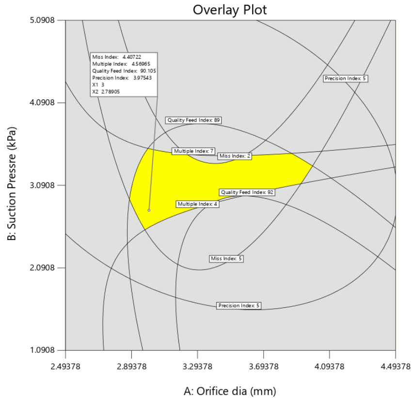
Fig.3 Overlay plot between orifice size and suction pressure
