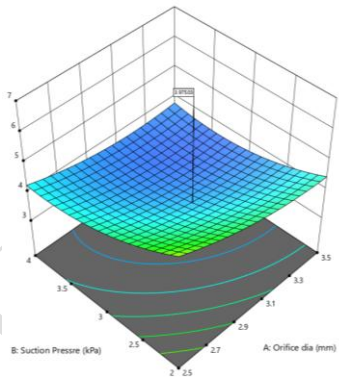
Fig.2 Comparison of different performance indices (level of significance, 5%): (a) miss index; (b) multiple index; (c) quality of feed index (d) Precision index for Orifice size x Suction pressure (AB), Orifice size x Forward speed (AC), Suction pressure x Forward speed.
