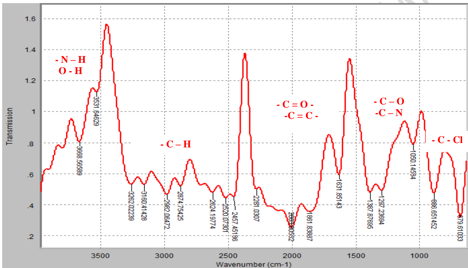
Figure 2: FTIR spectral profile of biosynthesized silver nanoparticles
