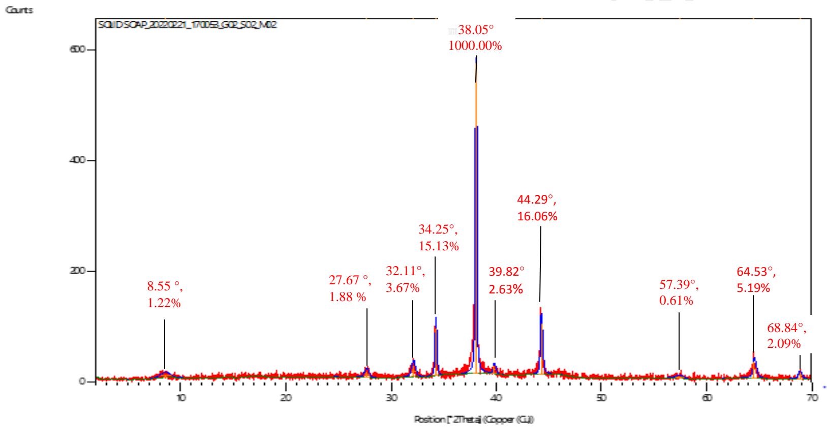
Figure 3: XRD profile pattern of the biosynthesized AgNPs
