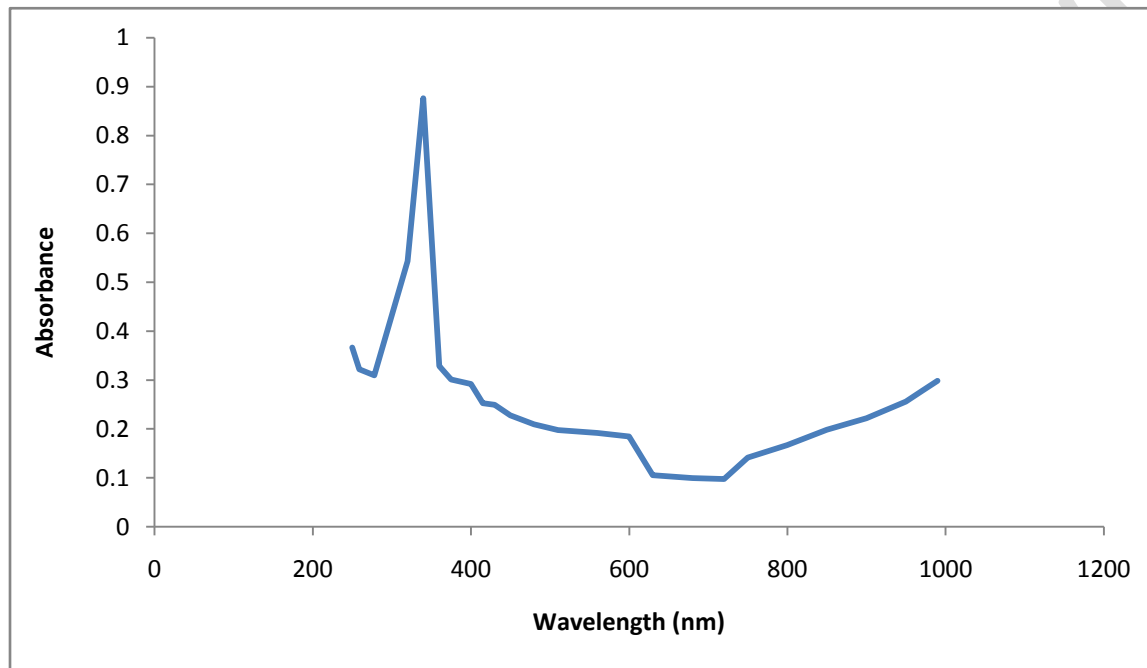
Figure 1: UV – Vis Absorbance spectral profile of silver nanoparticle
