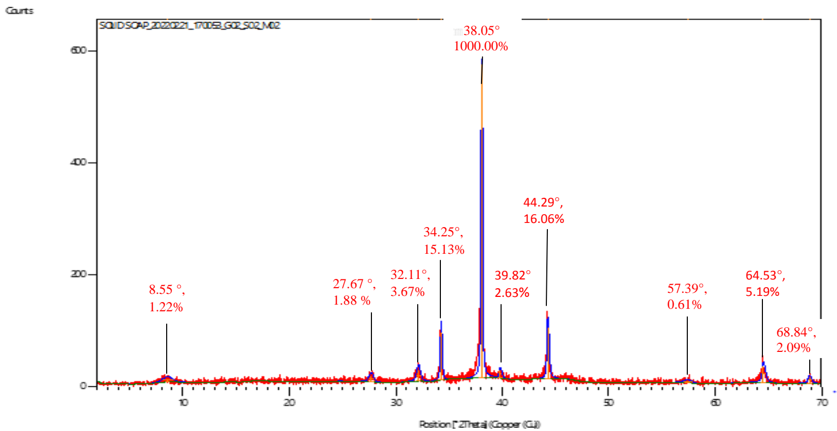
Figure 3: XRD profile pattern of the biosynthesized AgNPs
