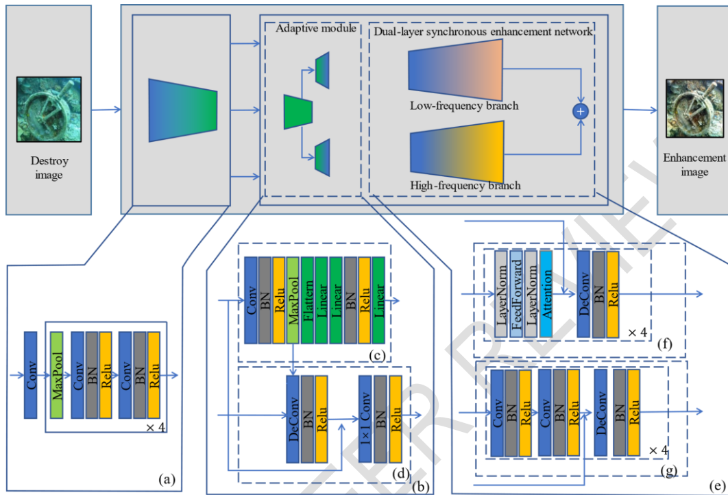
Figure. 1. The framework consists of three parts: (a) the encoder consists of a series of convolutional blocks; (b) an adaptive module consists of (c) water type classifier and (d) water type related feature extractor, which be used to separate the interference of water types; (e) a dual-layer synchronization network consists of (f) low-frequency branch and (g) high-frequency branch for learning high-frequency and low-frequency information separately.
