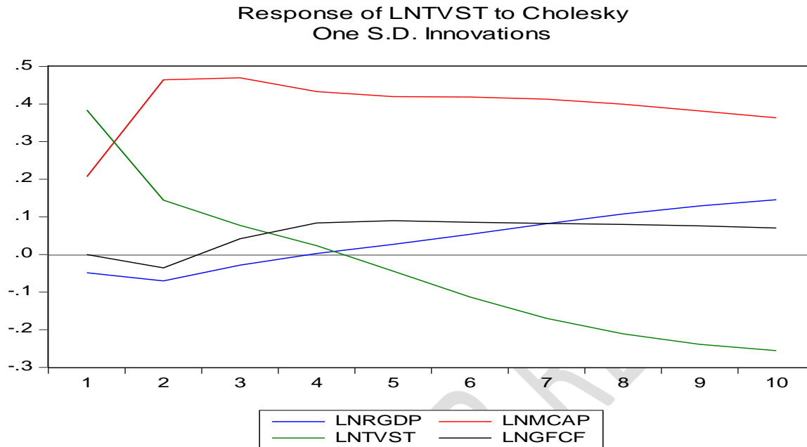
Figure 3: Combined Impulse Response Function of LNTVST to Cholesky One Standard Deviation Innovation
