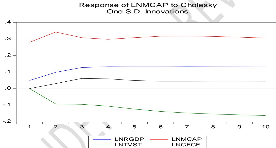
Figure 2: Combined Impulse Response Function of LNMCAP to Cholesky One Standard Deviation Innovation
