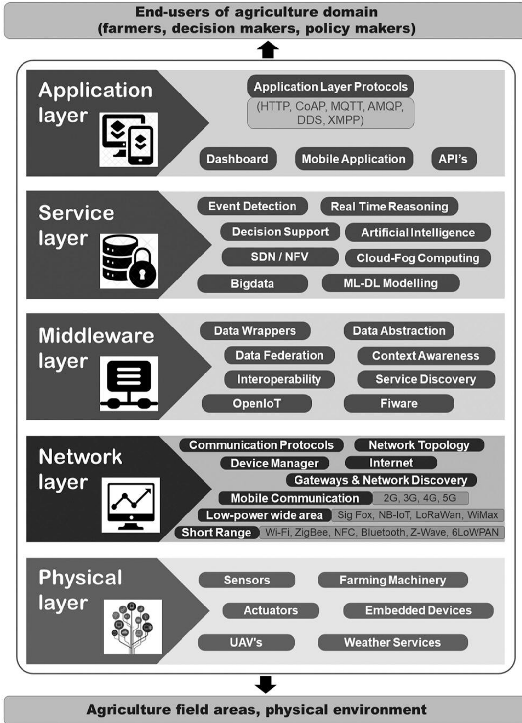
Fig 1.-Layered architecture of agriculture internet of things[7].
