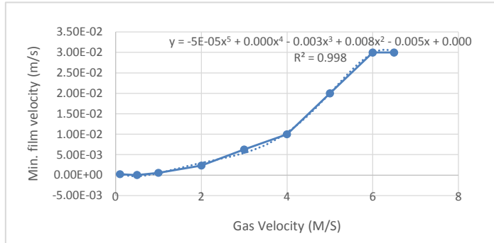
Figure 6: Relationship between minimum film velocity and superficial gas velocity at V_{sl} = 0.05 m/s
