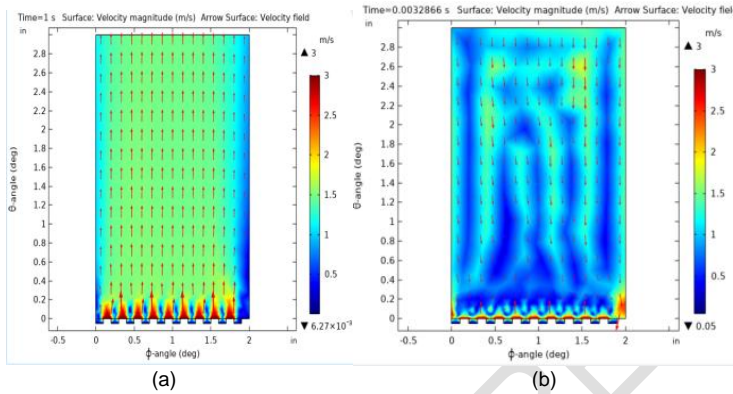
Figure 8: Simulation of annular flow regime at varying initial inlet conditions
