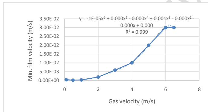
Figure 7: Relationship between minimum film velocity and superficial gas velocity at V_{sl} = 0.05 m/s
