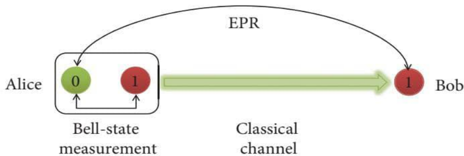
Figure 3: Illustration of the quantum teleportation model
