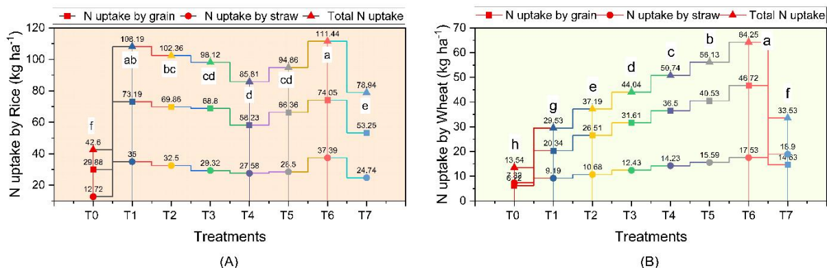
Fig. 6. Effect of organic and inorganic fertilizers on N uptake by rice and wheat (Data are mean, n = 3 ; p \leq 0.05 ), significant over control.
