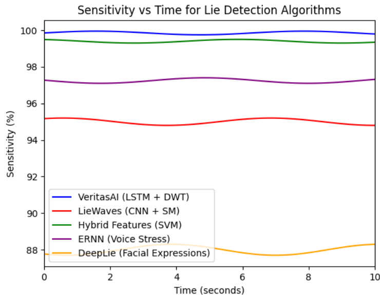
Fig.4. Graph for Sensitivity (%) versus Time (seconds)
