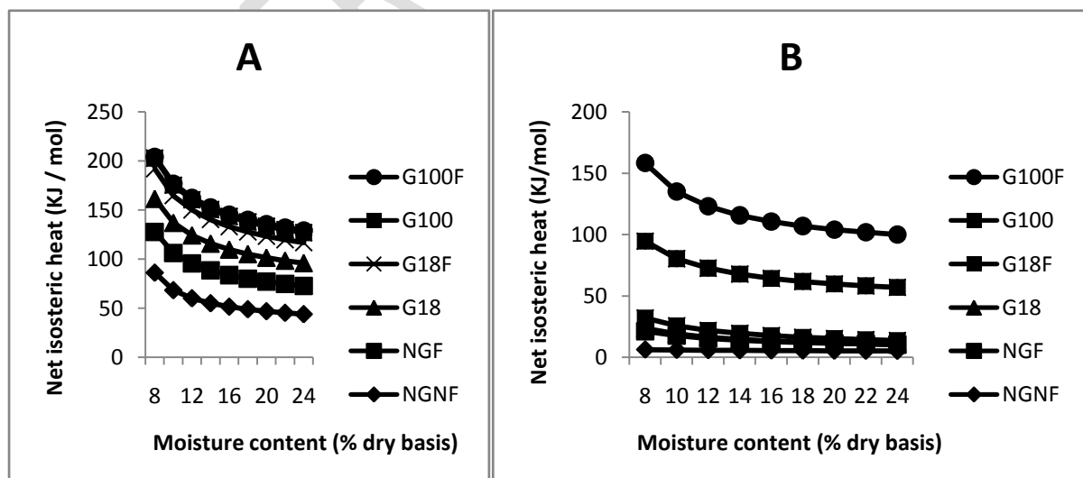
Figure 4: Isotheric heat of sorption for adsorption (A) and desorption (B) of plantain and soybean complementary foods.
