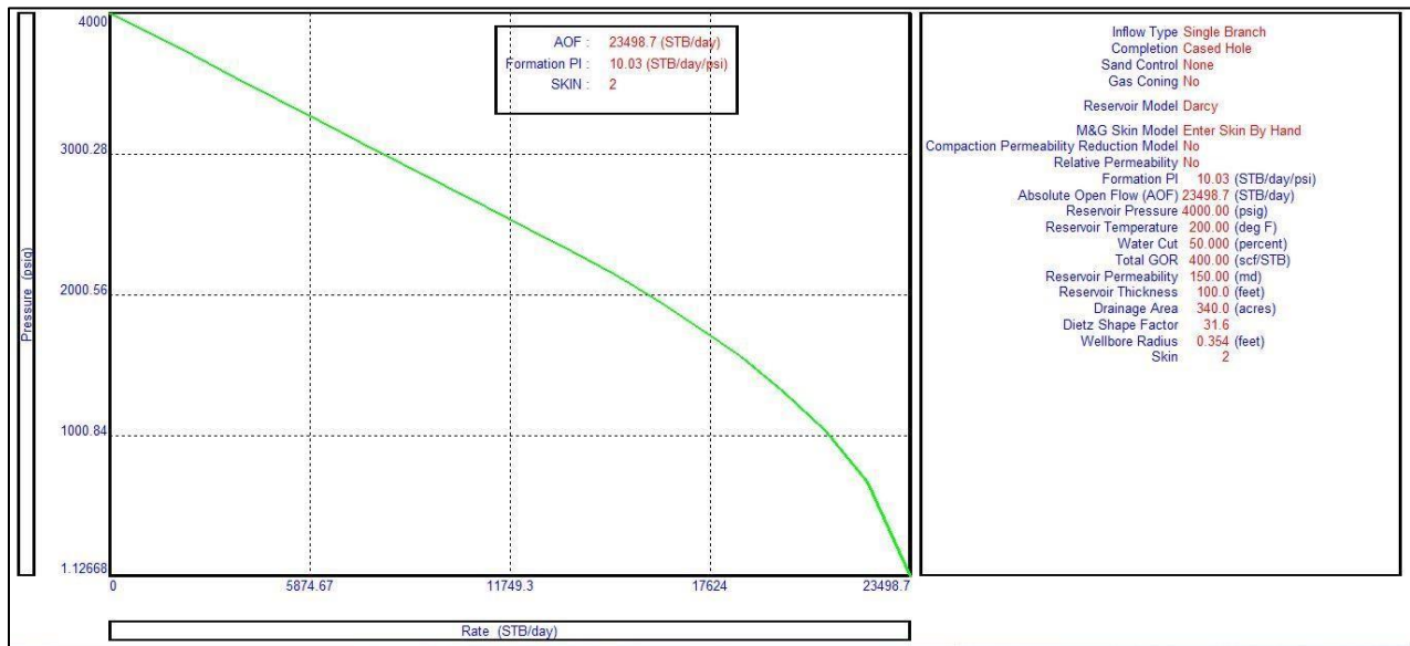
Figure 2: IPR curve for the well
