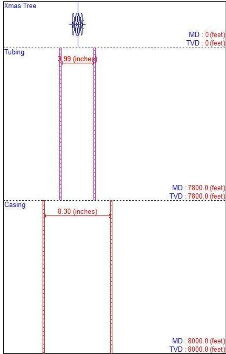
Figure 1: Down-hole architecture of well
