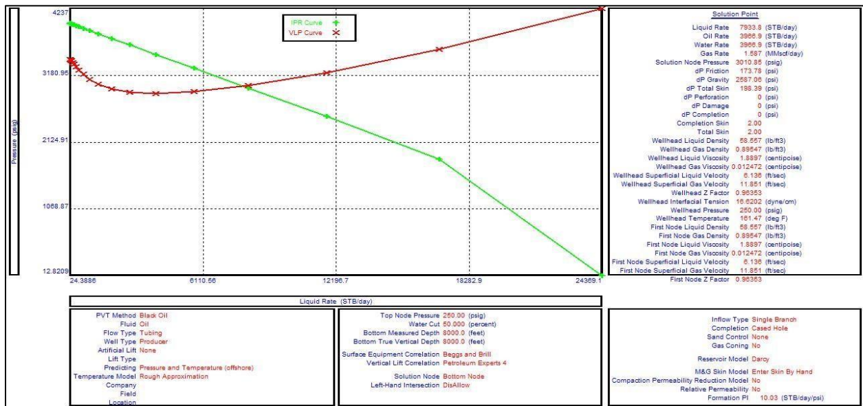
Figure 3: IPR-VLP curve for the well at a GOR of 400scf/stb
