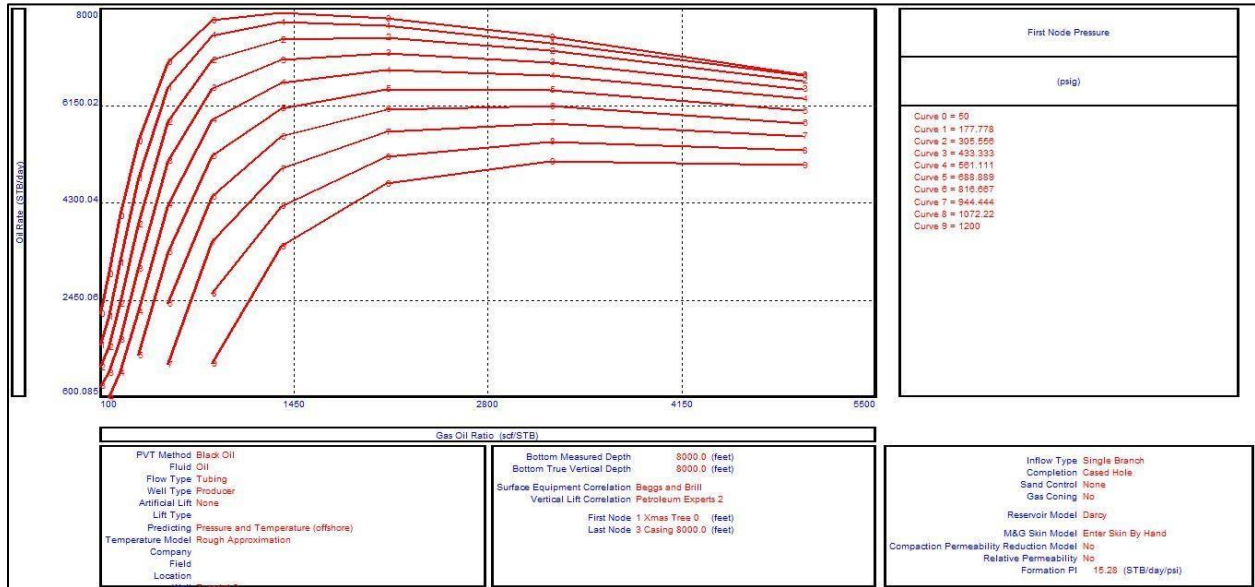
Figure 4: Sensitivity analysis showing a variation of oil rate with gas-oil ratio at different well head pressures
