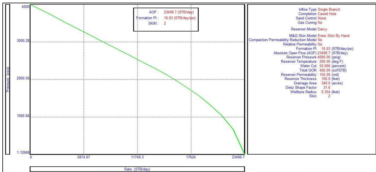
Figure 2: IPR curve for the well
