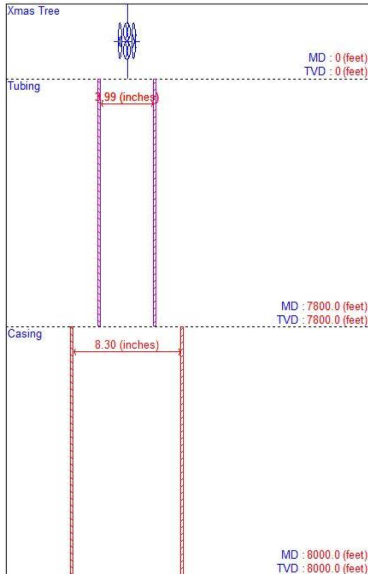
Figure 1: Downhole architecture of well
