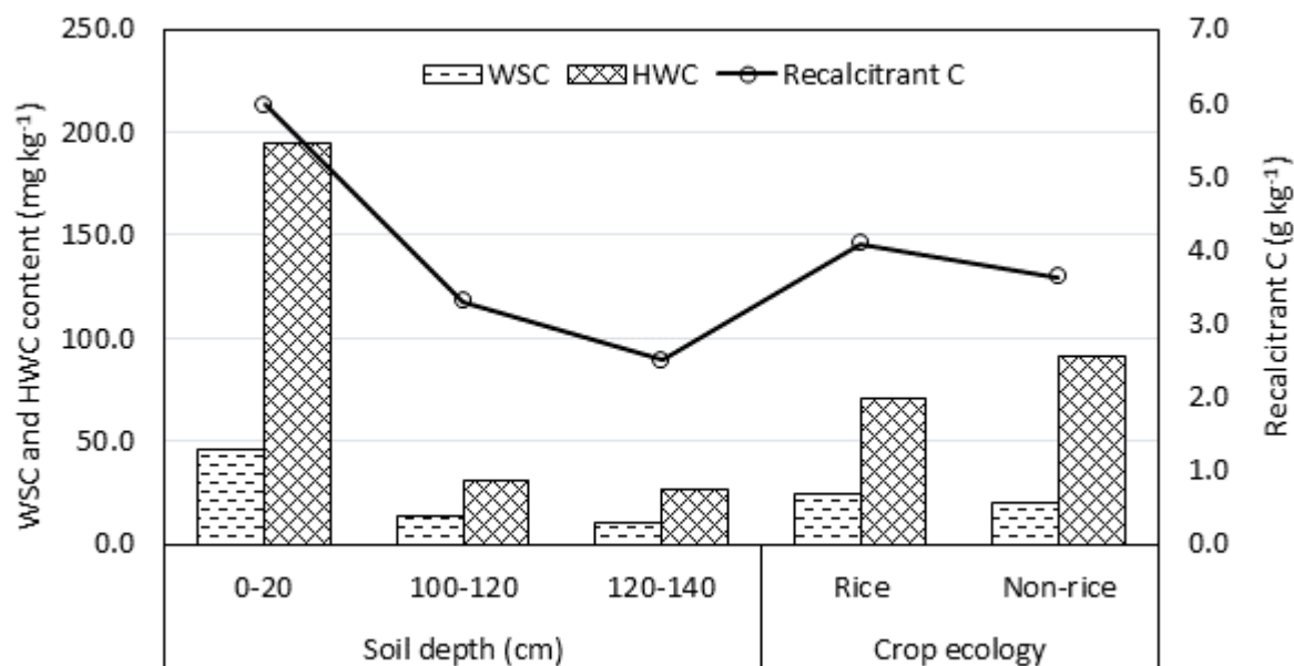
Fig 2. Status of water-soluble C (WSC), hot water-soluble C (HWC), recalcitrant C at different soil depth and crop ecology
