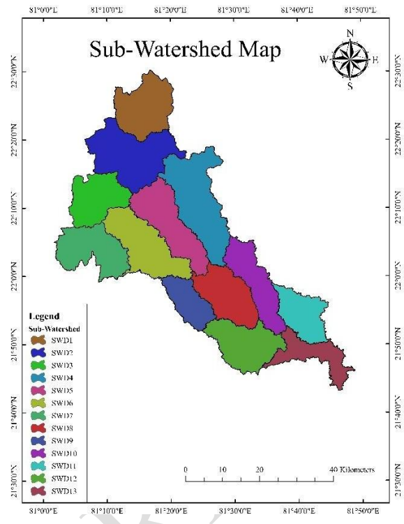
Fig. 4: Sub-watershed map Nawagarhwatershed
