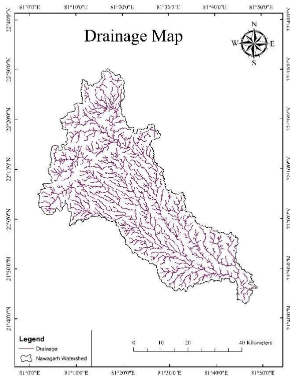
Fig.3: Drainagemap ofthe ofNawagarhwatershed
