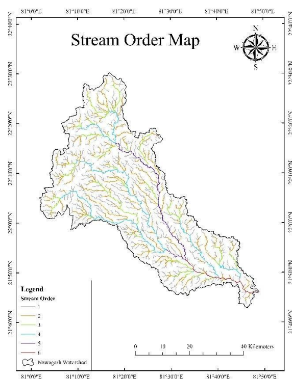
Fig. 6: Stream order map of Nawagarh Watershed
