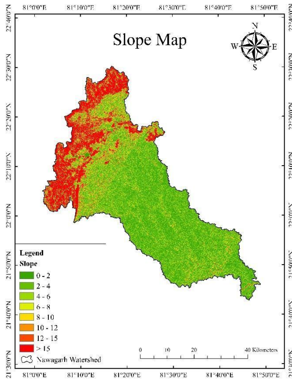
Fig.5: Slope map of the Nawagarh Watershed
