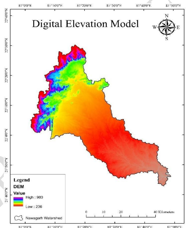
Fig.2: DEM of Nawagarh Watershed
