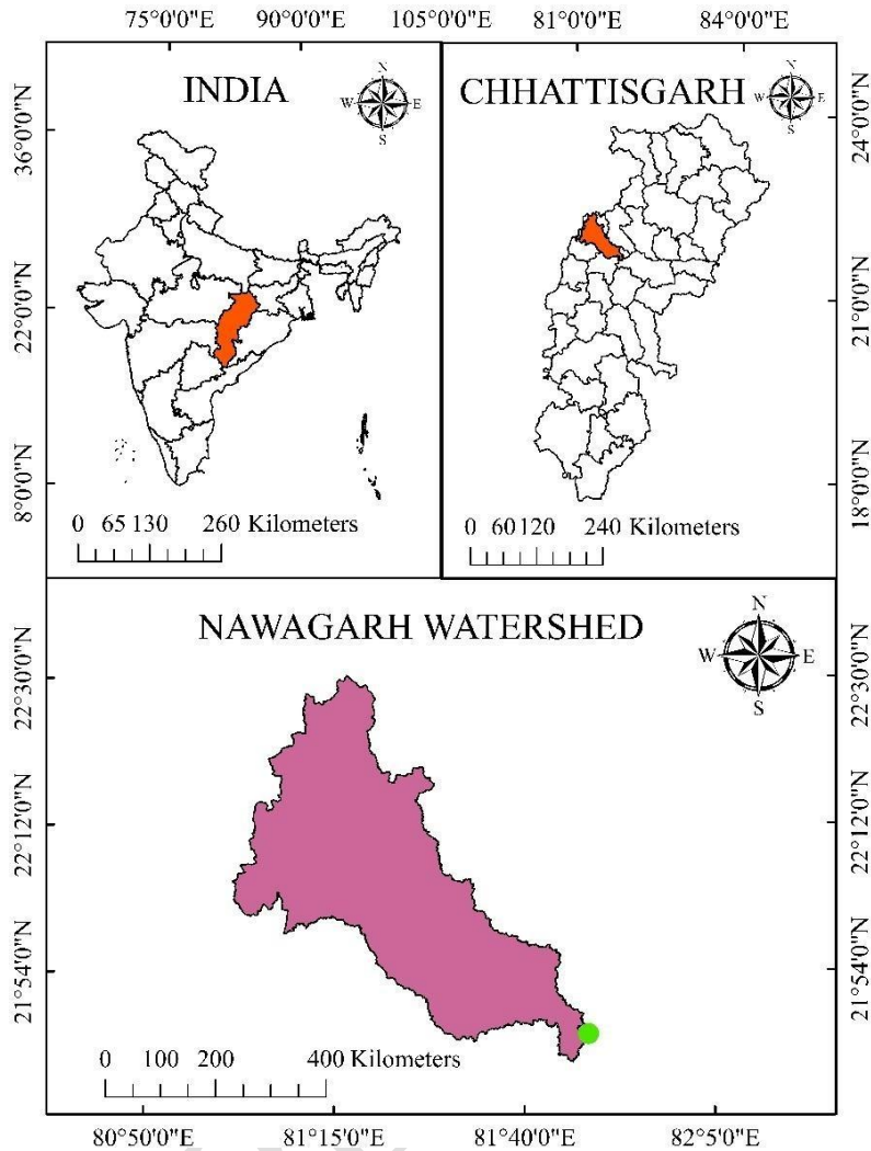
Fig.1: Location of Nawagarh Watershed
