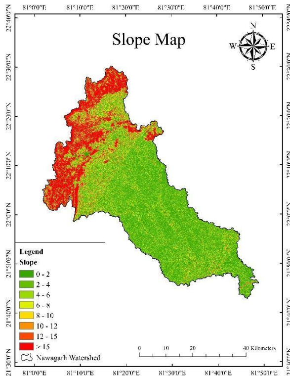
Fig.5: Slope map of the Nawagarh Watershed
