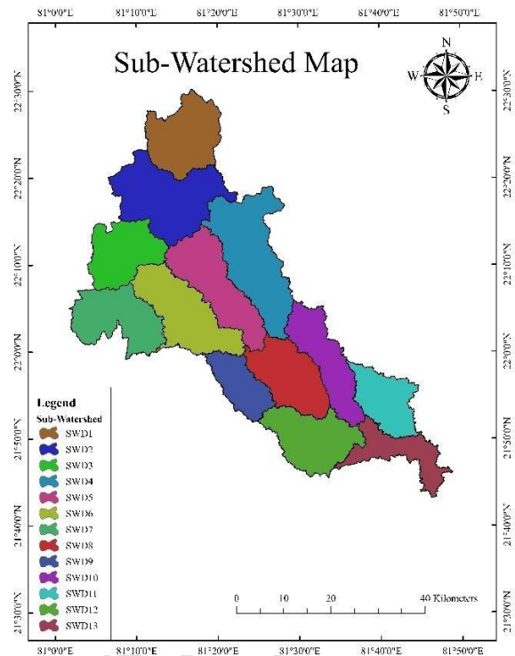
Fig. 4: Sub-watershed map Nawagarhwatershed
