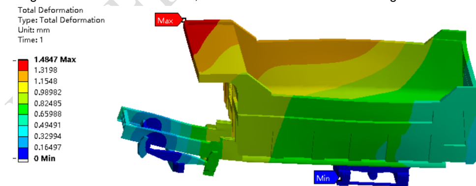
Figure 9. Total deformation cloud image
