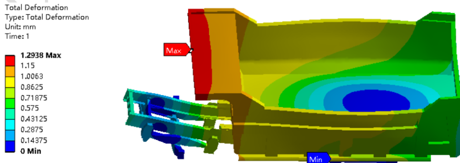
Figure 7.Total deformation cloud image
