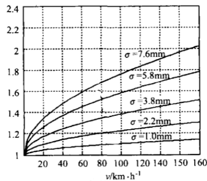
Figure 2. Selection diagram of dynamic load coefficient
