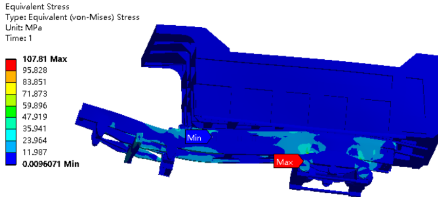
Figure 10. Stress nephogram
