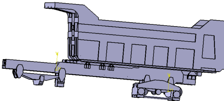
Figure.1.Body structure of the frame
