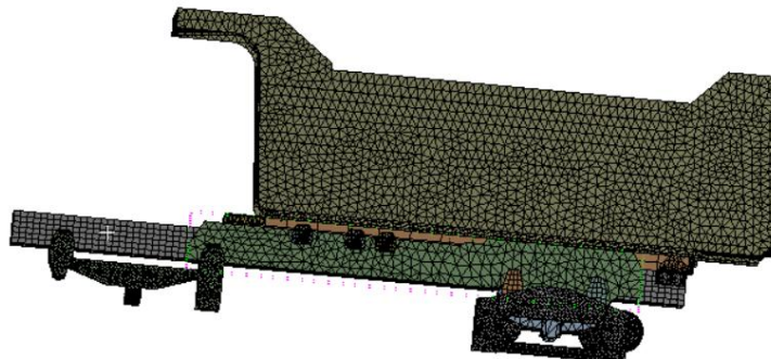
Figure 4. Meshing diagram
