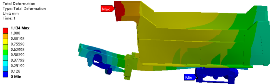
Figure 5.Total deformation cloud image
