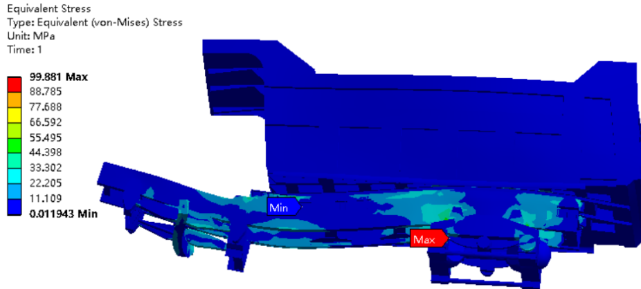
Figure 8. Stress nephogram
