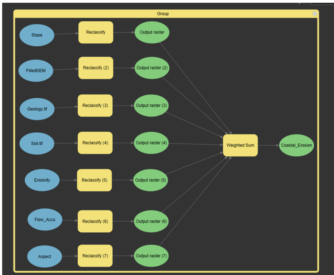
Figure 2: Coastal Erosion Vulnerability Graphic Model
