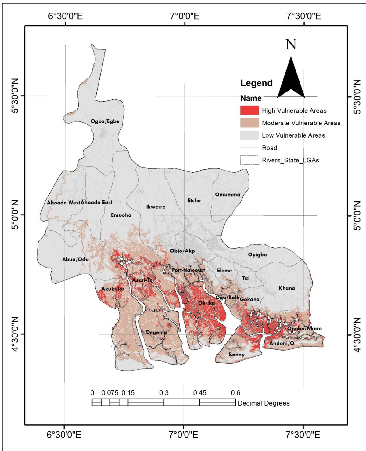
Figure 4: Coastal Erosion Vulnerability in Rivers State, Nigeria
