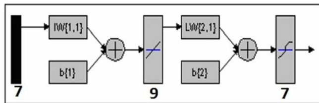
Figure 2- Neural network design used in research
