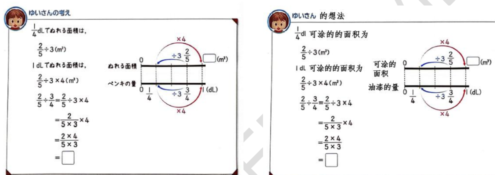
Figure 8 The example of Deductive reasoning supplemented by intuitive geometry wall painted by 1 liter of paint is 2/15 × 4 = 8/15.
