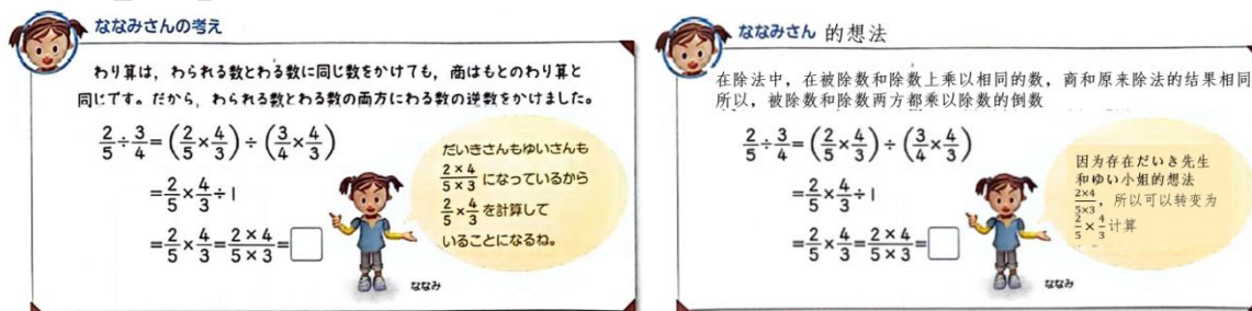
Figure 9 The example of Deductive reasoning
