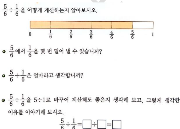
Figure 5 The example of The intuitive geometry
