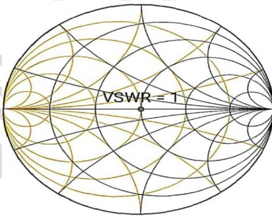
Fig.4: Smith Chart of the Impedance Matching
