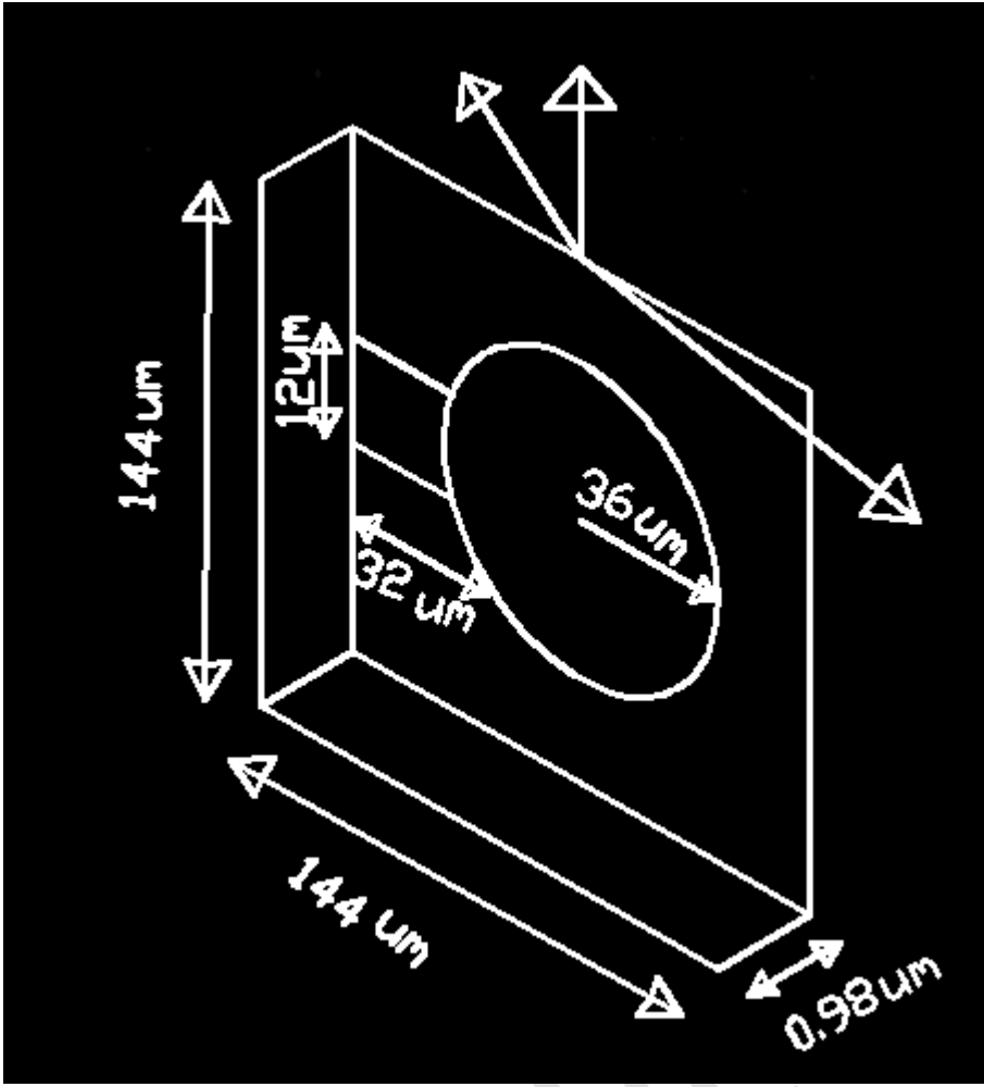
Fig. 2: The proposed Circular Micro-strip Patch Antenna
