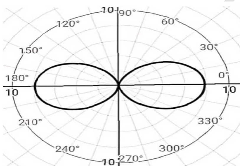
Fig. 6: The polar plot of the Antenna Radiation Pattern in the Azimuth Angle of 0^\circ and 180^\circ .
