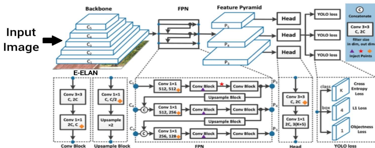
Fig. 1. Architecture of YOLOv7
