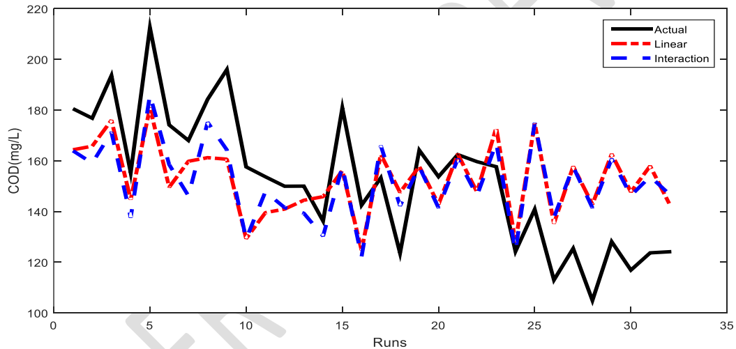
Figure 3; COD RSM prediction comparative plot
