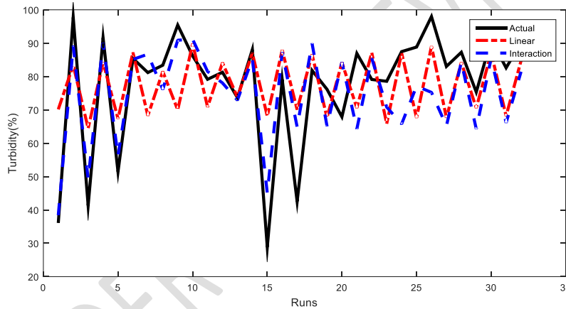
Figure 4; Turbidity RSM prediction comparative plot
