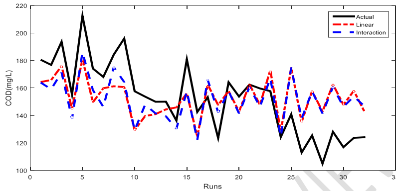
Figure 3; COD RSM prediction comparative plot
