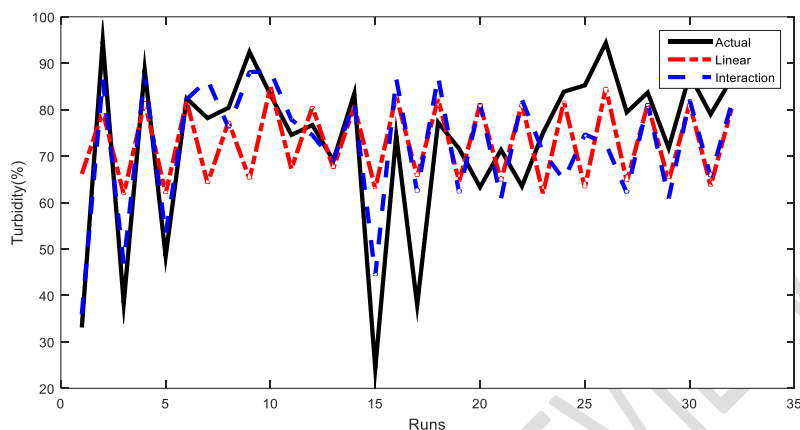
Figure 5; Colour RSM prediction comparative plot
