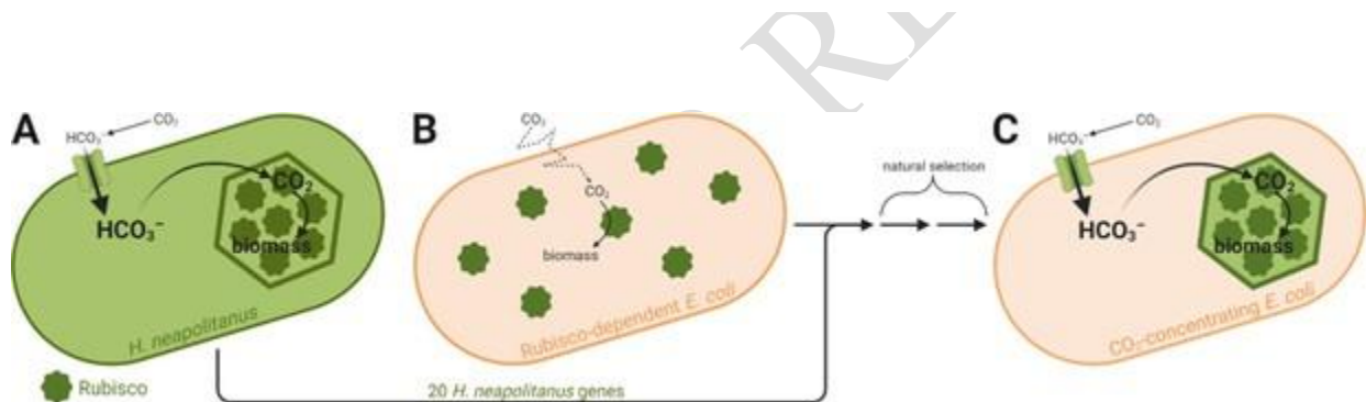
• Figure 1. Engineering a carbon-concentration into E. coli
