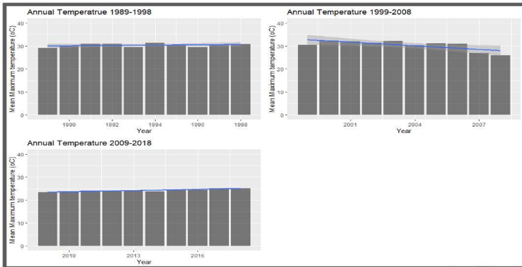
Figure 5b: Annual temperature trends in RUNAPA from the 1980s-2018. Source: Field survey data, (2021).
