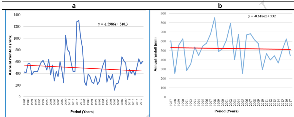
Figure 3: Annual rainfall trends in RRL; a) RGRs from the 1980s-2018 and b) RUNAPA from the 1980s-2018. Source: Field survey data, (2021).
