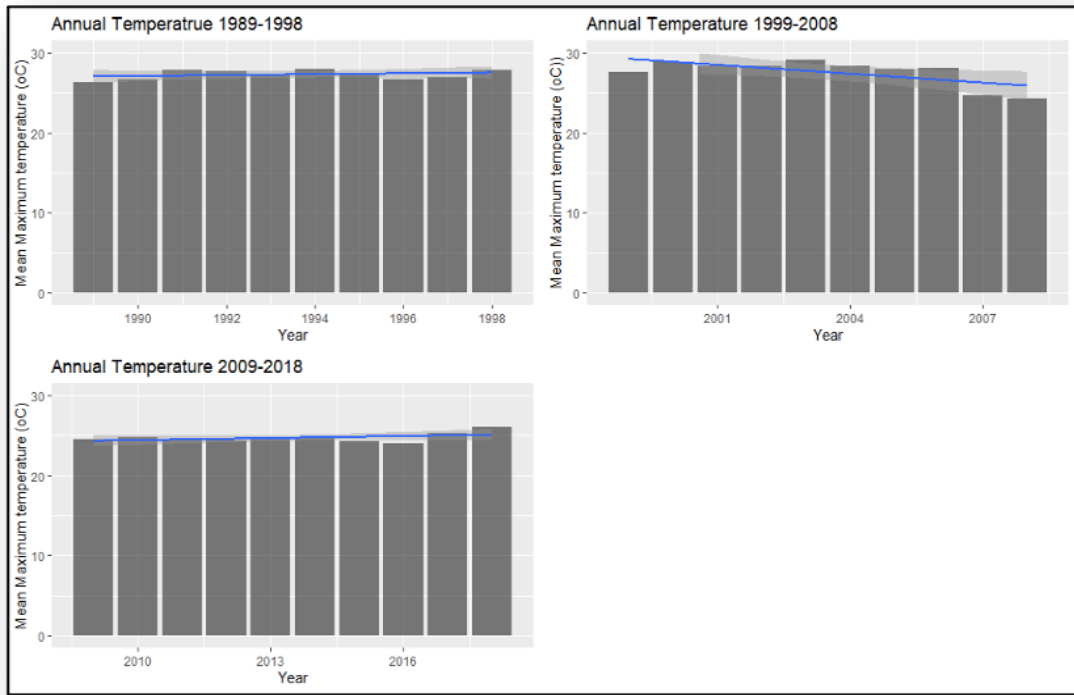
Figure 5a: Annual temperature trends in RGRs from the 1980s-2018. Source: Field survey data, (2021).
