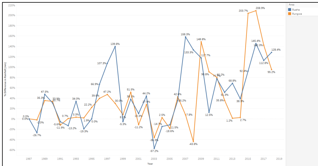
Figure 4: Percentage difference of rainfall received in RUNAPA and RGRs, 1980s-2018. Source: Field Data Collection, (2021).
