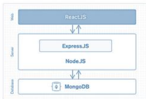
Figure 3: Technology stack.
