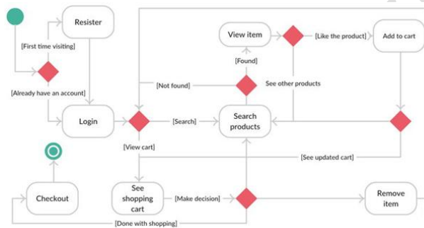
Figure 7. State flow Diagram.
