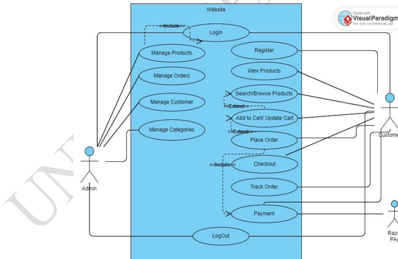
Figure 5. UML diagram for Nandini chicken
