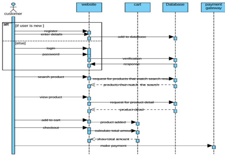
Figure 6. Sequence diagram for Nandini chicken
