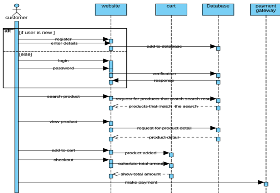
Figure 6. Sequence diagram for Nandini chicken
