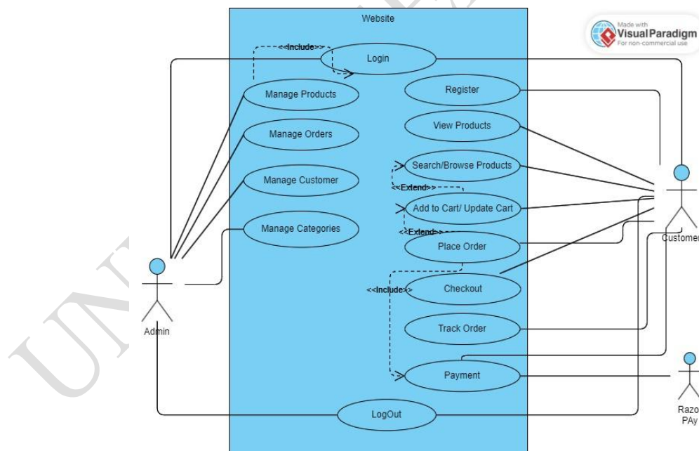
Figure 5. UML diagram for Nandini chicken
