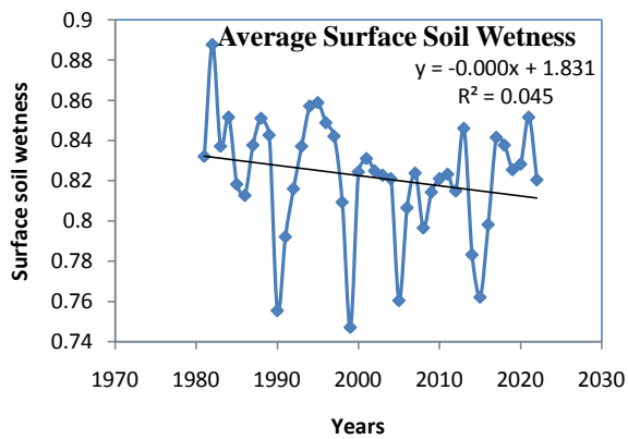
Fig. 5: Mean surface soil wetness (SSW)
