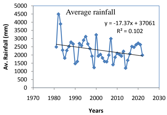
Fig. 3: Average Rainfall Variations
