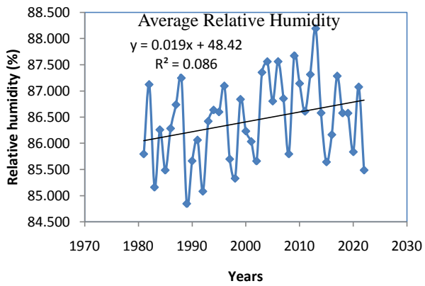
Fig. 4: Average relative humidity variations
