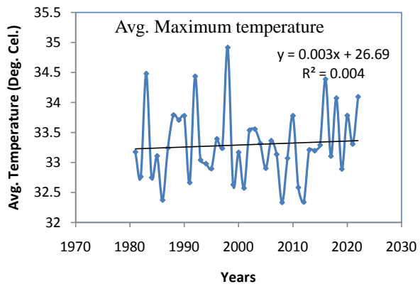
Fig. 2: Average maximum temperature variations.
