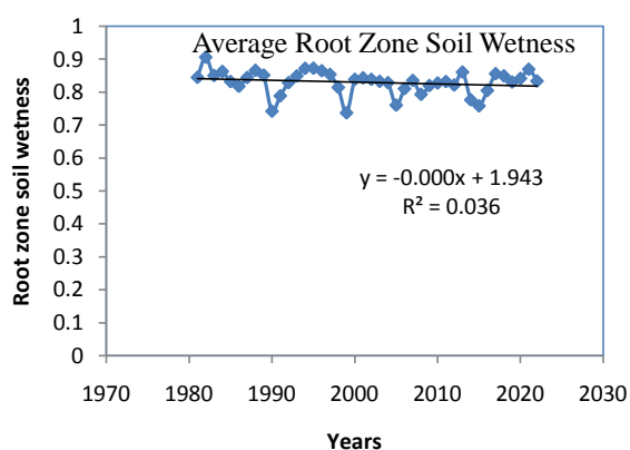
Fig 6: Mean Root Zone Soil Wetness (RZSW)
