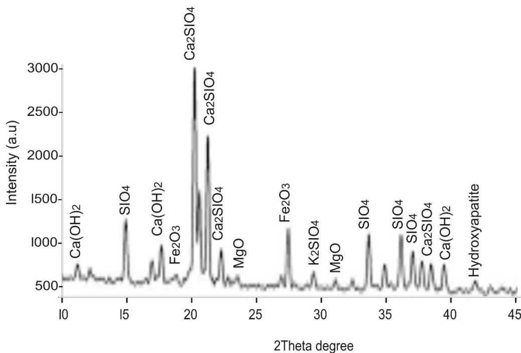
Fig8. Rice Husk Calcined at 600 °C (KD)
