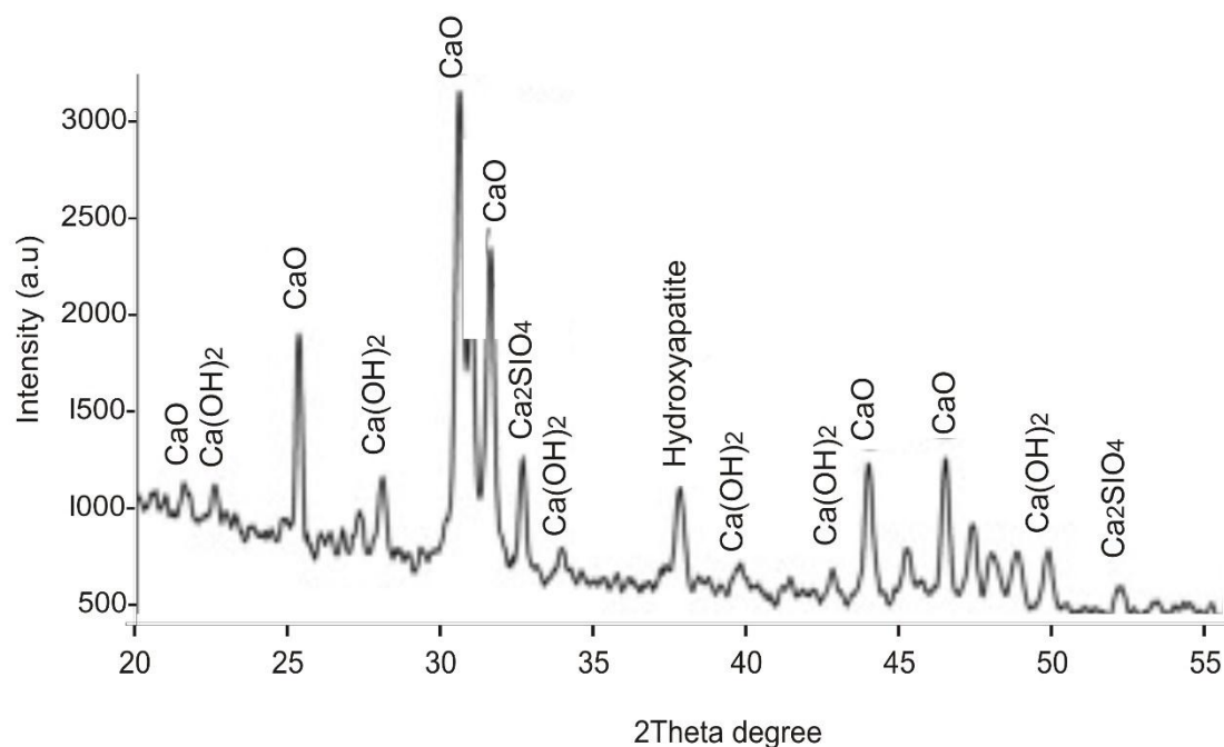
Fig7 Eggshell Calcined at 700 °C (KC)
