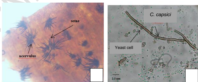
Figure 5. (A) symptom of anthracnose disease by Colletotrichum capsici on chili fruit, (B) The relationship between antagonistic yeast and C. capsici
