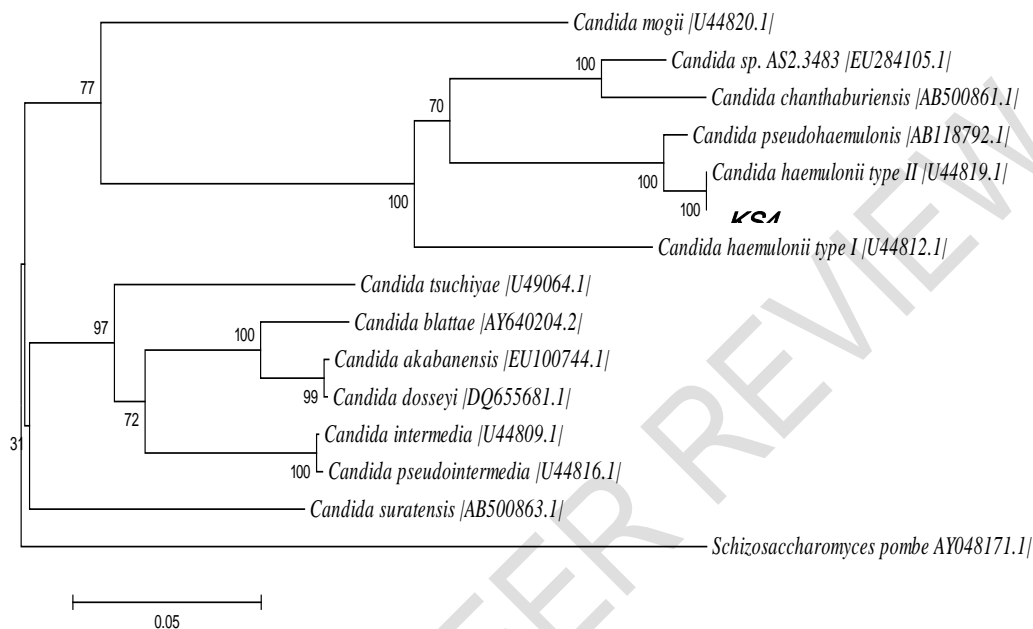
Figure 6. Phylogenetic tree of KS46 with respect to closely related species based on the sequence of the D1/D2 domain, using the neighbor-joining method. Numbers indicate percentages of bootstrap sampling, derived from 1,000 samples.
