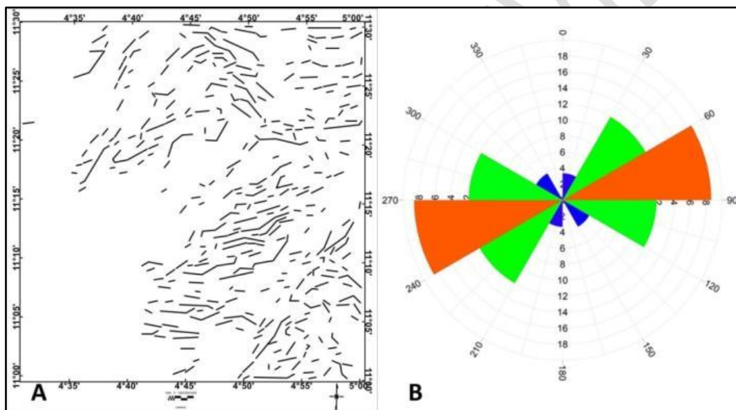
Figure 7: a. Structures from FVD Map b. Rose Diagram from FVD Structures
