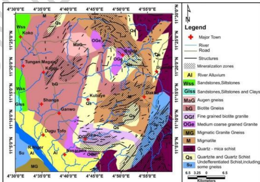
Figure 12: Integration of Shanga Structures with the Geology (NGSA, 2009)
