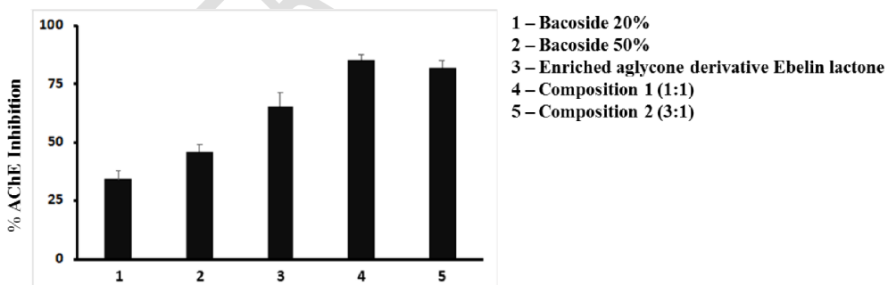
Figure 2: Graph representing the percentage of Acetylcholinesterase inhibition for various Bacopa Herbal Compositions
